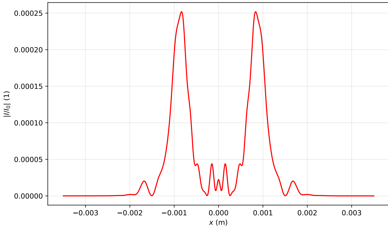
Intensity profile I(x, y = 0, z = 1.035)/I_0 , P_{in}=7.0P_{cr} , artificial time
